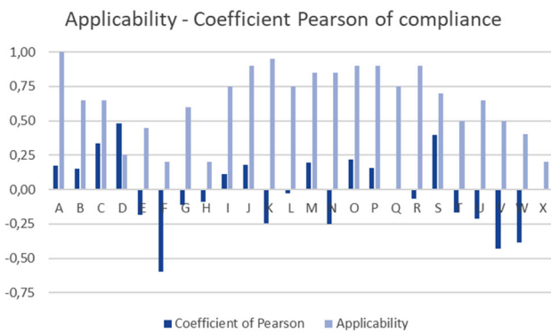
Fig. 42 Statically analysis of the applicability
