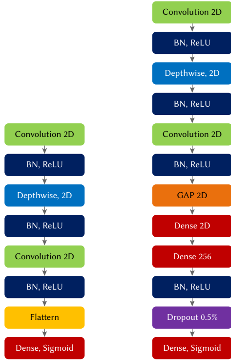
Fig. 2. (a) Core layers of MobileNetV2 (b) Core layers of Modified MobileNetV2 (MpoNet).
