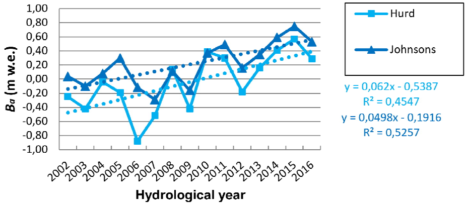
Fig. 7. Temporal evolution of the annual climatic mass balance of Hurd and Johnsons glaciers over the study period 2002-2016, together with their linear least-square fits. The p-values of the regression straight lines are 0.0058 for Hurd and 0.0022 for Johnsons.
