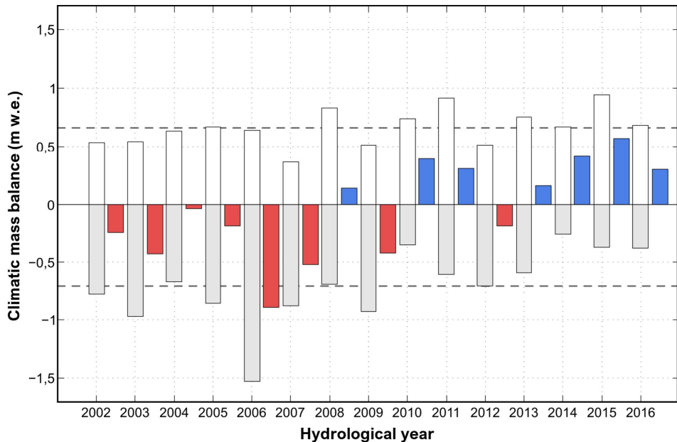
Fig. 4. Glacier-wide climatic mass balance of Hurd glacier for the hydrological years 2002–2016, calculated using the glaciological method and a specific DEM and glacier outlines for each individual year within the study period. For each year, the white bar represents the winter balance, B_w , the grey bar the summer balance, B_s , and the blue or red bar to the right of the white/grey bars the resulting annual balance, B_a , shown in blue if positive, and in red if negative. The dashed horizontal lines represent the means of the winter (positive values) and summer (negative values) balances.
