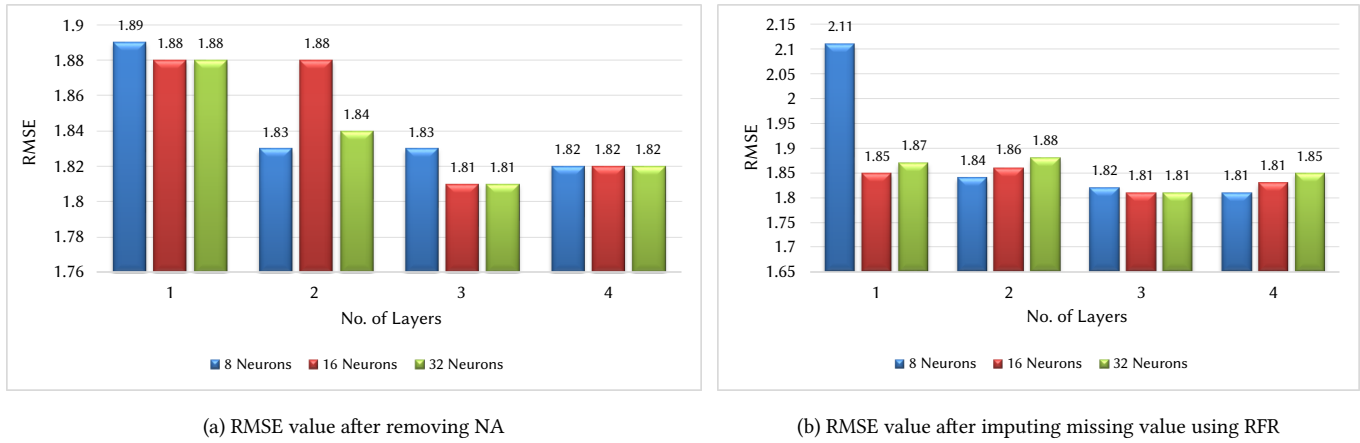
Fig. 8. RMSE value of Sotavento wind farm dataset
