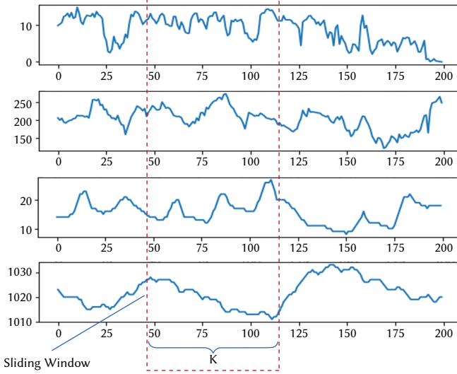
Fig. 2. Sliding Window.
