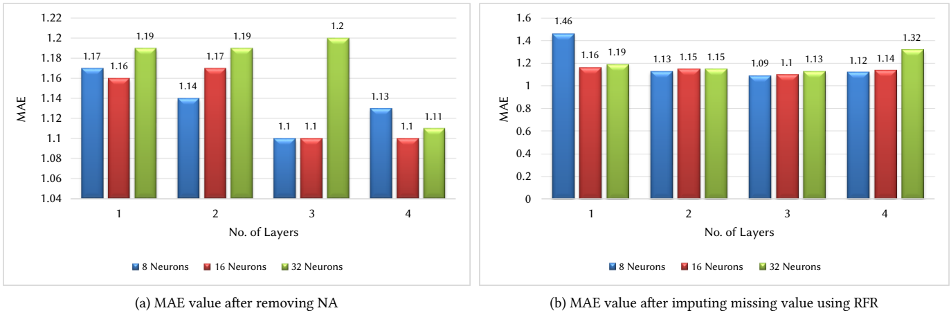
Fig. 7. MAE value of Sotavento wind farm dataset.
