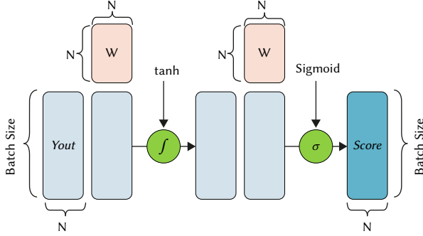
Fig. 4. Attention procedure over Features.
