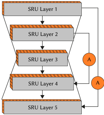
Fig. 3. The proposed SRU architecture.
