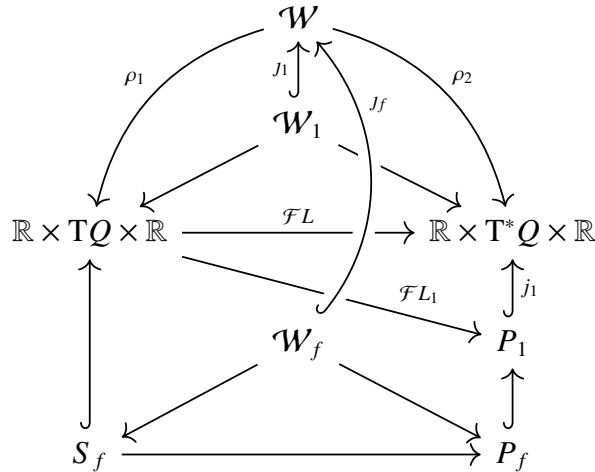
Figure 1. Recovering the Lagrangian and Hamiltonian formalisms.
