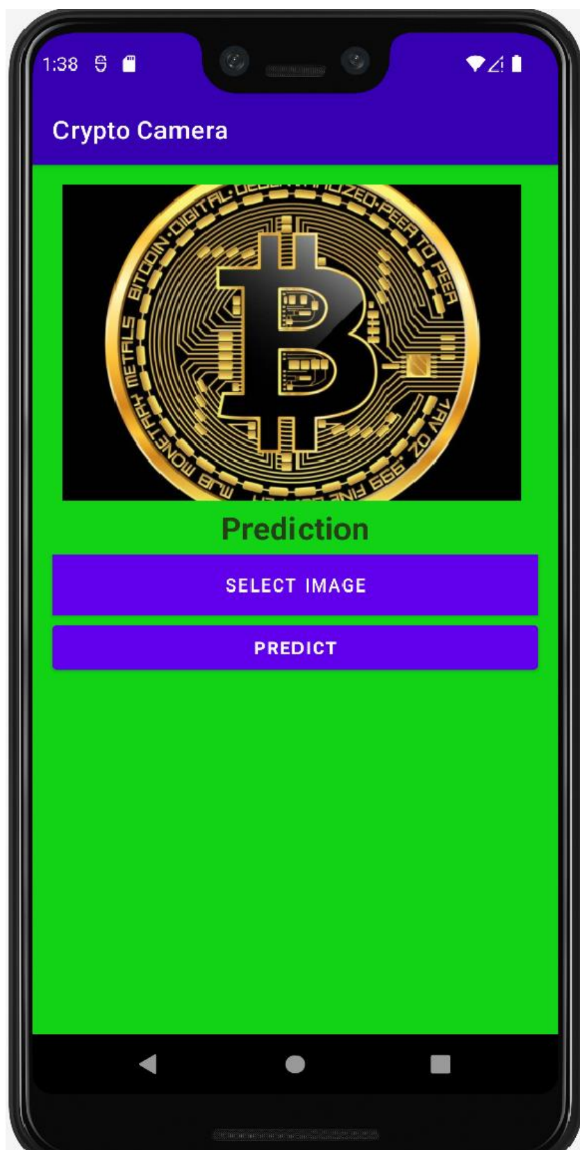
(Interfaz-Prediction)
