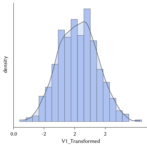
Fig. 3. Histogram for the transformed variable.
