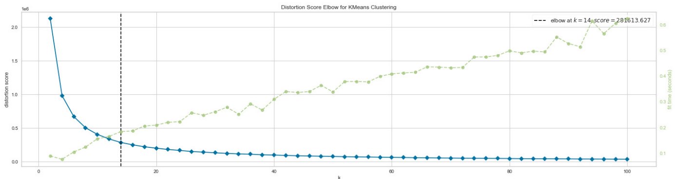
Fig. 8. Results of the elbow method for the number semantic clusters of hashtags.
