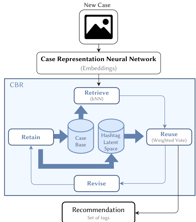
Fig. 2. Overview of the proposed CBR-based recommender system.
