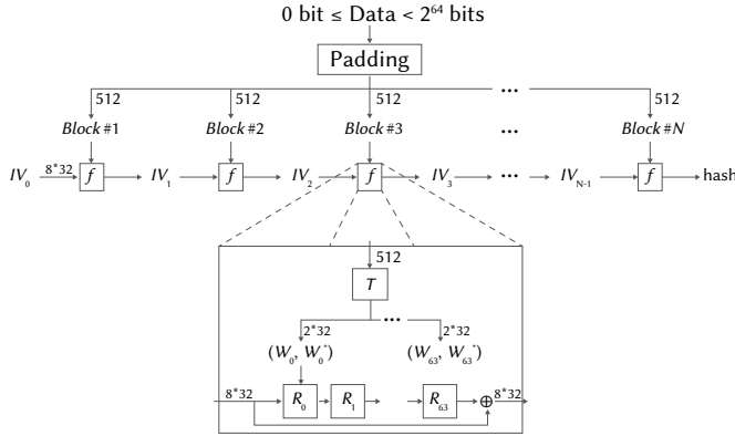
Fig. 1. Structure of SM3 algorithm.
