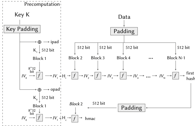
Fig. 3. Structure of HMAC SM3.
