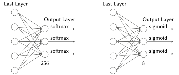
Fig. 7. The difference of output layers between CNN best and CNN multi-label . Left: the output layer of CNN best . Right: the output layer of CNN multi-label .
