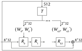
Fig. 2. Structure of the f function.
