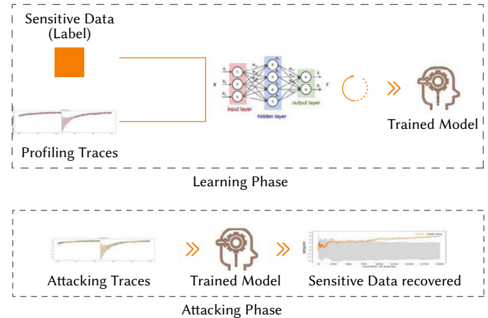
Fig. 5. The procedure of deep learning-based side channel analysis.
