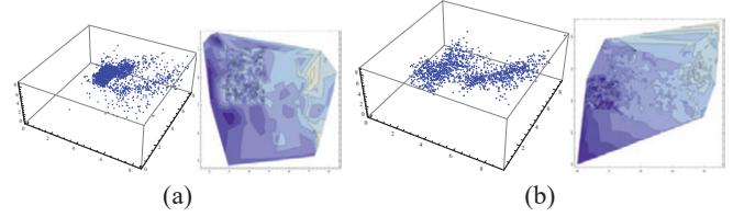
Fig. 2. The density distribution (middle) and contour map (right) of the linear density function of the VAD spatial point, where (a) K=control, and (b) K=modern.
