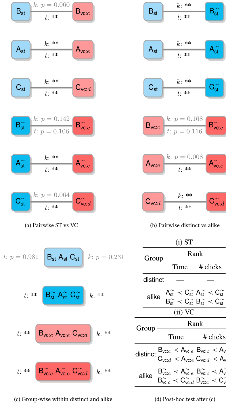
Fig. 8. Diagrams of the statistical tests performed on comparing types of puzzles (a, b) pairwise (Mann-Whitney rank test) and (c) group-wise (Kruskal-Wallis H-test), for completion time ( t ) and number of clicks ( k ). Bonferroni correction is applied with \alpha^* = 0.05/m , for m = 48 accounting for the all pair-wise hypotheses (24) and the two dependent variables ( t and k ). Note: ** means p -value is very low (lower than 0.0001), thus representing statistically significant differences (d) Ranking puzzles from pair-wise post-hoc tests (Mann-Whitney rank test). Note: the notation X < Y represents that significant differences exists between X and Y and puzzle X has lower mean for the corresponding metric than puzzle Y .
