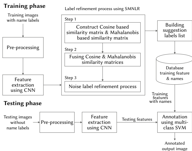
Fig. 1. Process flow of the proposed SMNLR method.
