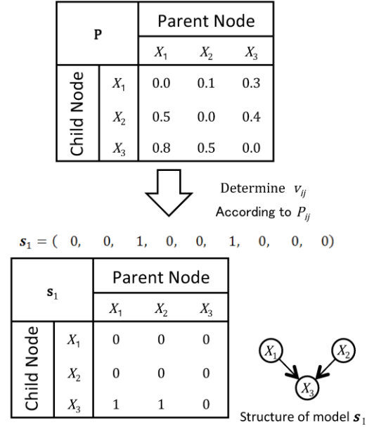
Fig. 3. Step (2): Generating Individuals
