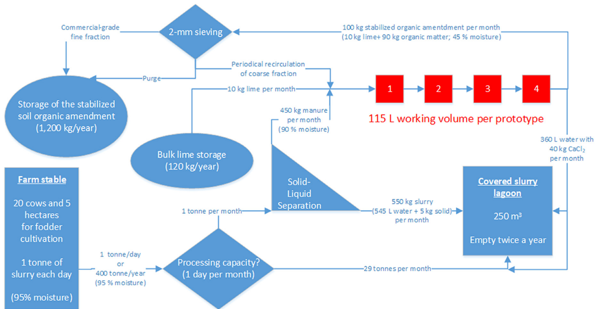
Fig. 6. Operation of 4 prototypes at a small farm (i.e. 20 dairy cows).
