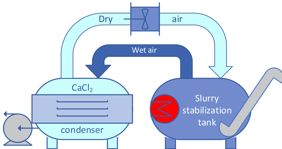
Fig. 1. Schematic of the prototype developed based on previous investigations (Moure Abelenda et al., 2022, 2021a,b,c; Moure Abelenda and Aiouache, 2022; Moure Abelenda and Amaechi, 2022).
