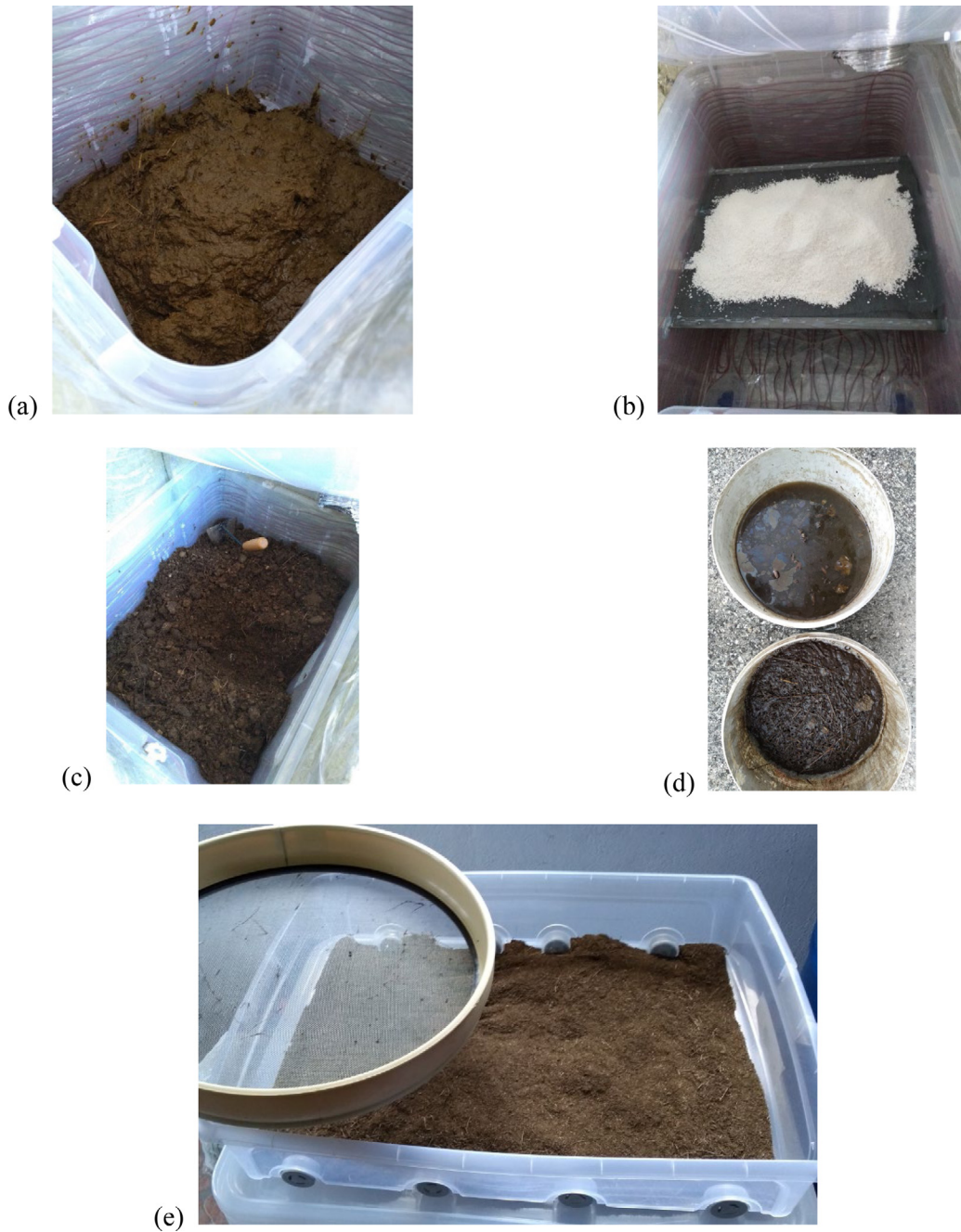
Fig. 4. (a) Fresh organic manure (90% moisture) in the 150-L stabilization chamber; (b) CaCl 2 in the tray of the condensation vessel; (c) stabilized manure after 2 weeks of operation (45% moisture); (d) testing the CaCl 2 -brine as additive of fresh slurry, which was generated in the condensate chamber, to avoid crust formation; (e) upgraded soil organic amendment (25% moisture) after 2-mm sieving.
