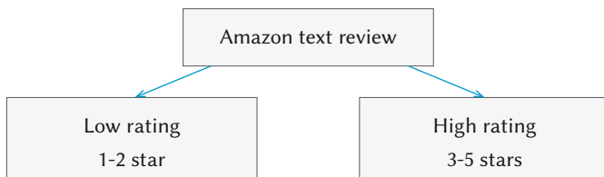
Fig. 2. Binary Classification.
