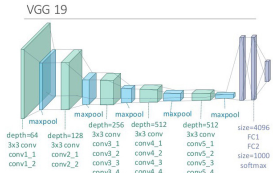
Fig. 1. VGG19 Model Architecture.
