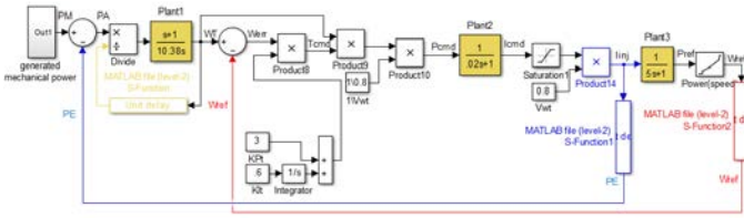
Fig. 5. The model of DFIG without using MOGA technique.
